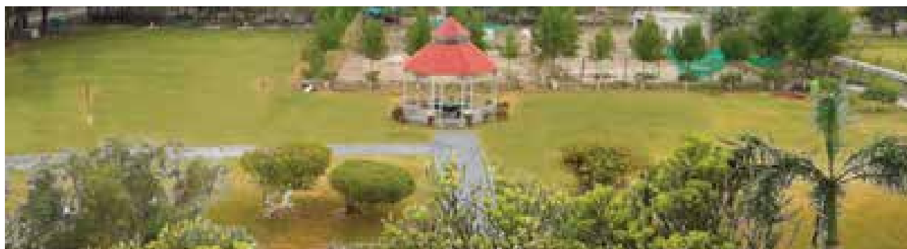
SCIL-Environment
